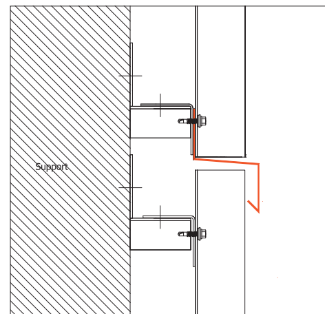
DRIP EDGE VERTICAL APPLICATION
